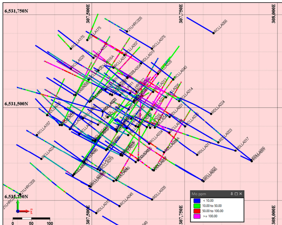
Figure 2. Moly (pink colour) in Central Porphyry sitting on edge of the main porphyry body.
